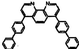
Structural formula 7:
